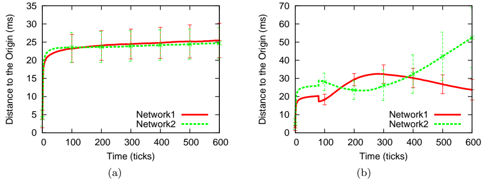
Fig. 12. The distance to the origin for the frog-boiling Network-Partition attack on the Kalman filter-based secure scheme with (a) no attackers, and (b) 10% attackers
